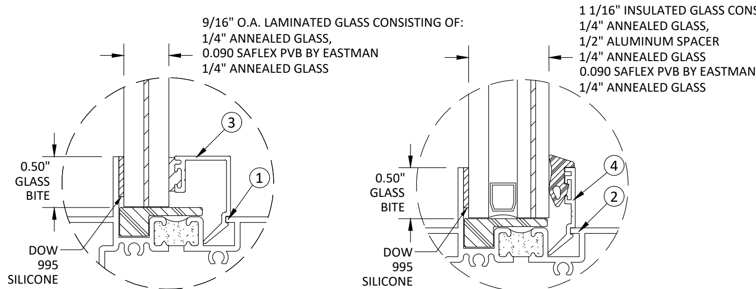
GLAZING DETAIL 1
