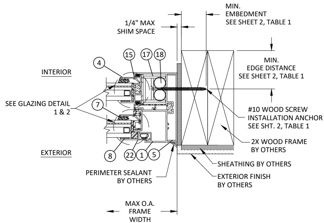
G 4 HORIZONTAL SECTION 2X WOOD BUCK SHEAR PLATE INSTALLATION
