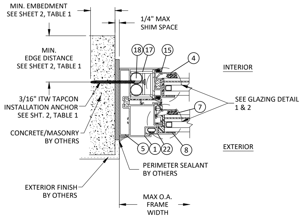
F 4 HORIZONTAL SECTION CONCRETE/MASONRY SHEAR PLATE INSTALLATION
